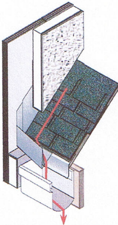
Figure 4: Diverter flashing at Roof / wall intersection
